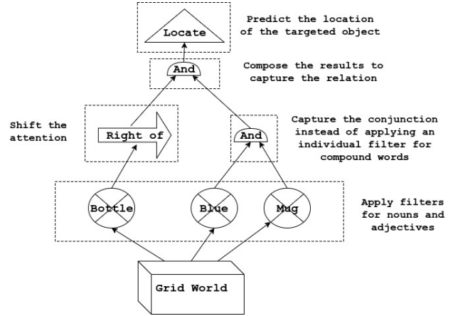
Figure 2: The layout generated for the instruction: “Pick the blue mug on the right of the bottle”.
