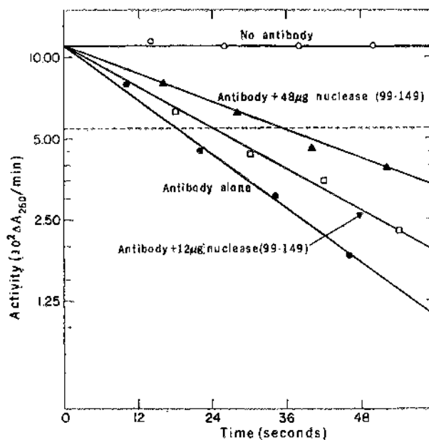
Fig. 12. Semilogarithmic plot of activity against time for assays of 0.05 \mu g of nuclease in the presence of: \circ — \circ , no antibody; \bullet — \bullet , 6 \mu g of antibody to (99 to 126) n ; \square — \square , 6 \mu g of antibody to (99 to 126) c plus 12 \mu g of (99 to 149); and \blacktriangle — \blacktriangle , 6 \mu g of antibody to (99 to 126) n plus 48 \mu g of (99 to 149). The dotted line represents one-half of the initial activity.
