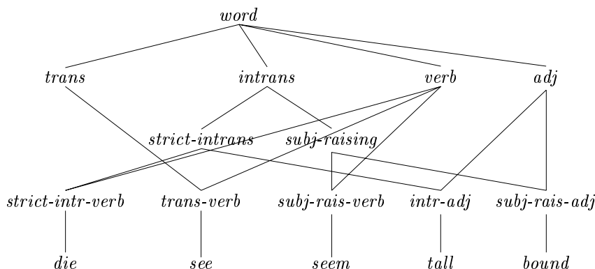
Figure 2: A simple hierarchy of words
