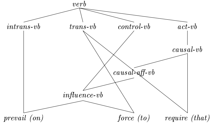
Figure 17: A multidimensional hierarchy of control verbs
