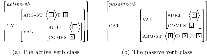
Figure 10: The active-vb and passive-vb verb classes
