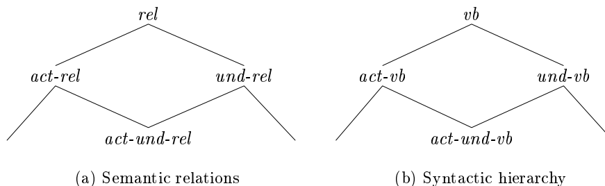
Figure 8: Homomorphism between semantic relation types and linking types
