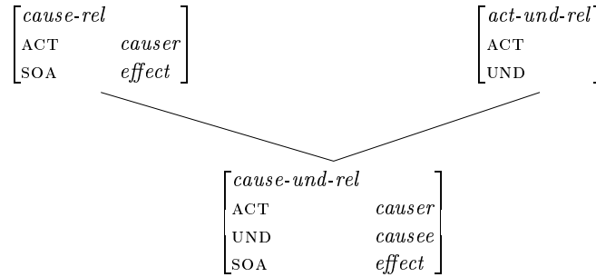
Figure 18: Two varieties of causal relations
