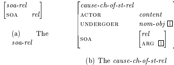
Figure 6: The soa-rel and cause-ch-of-st-rel relations
