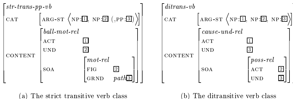
Figure 16: The strict transitive and ditransitive English verb classes for verbs of caused ballistic motion
