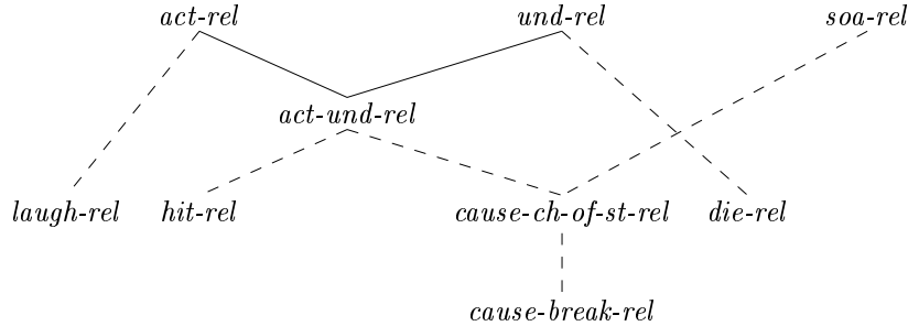
Figure 5: Classification of semantic relations using multiple inheritance
