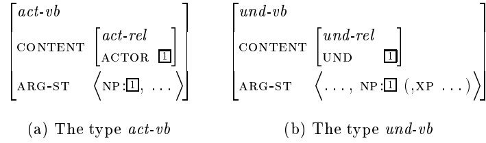
Figure 9: The act-vb and und-vb linking classes
