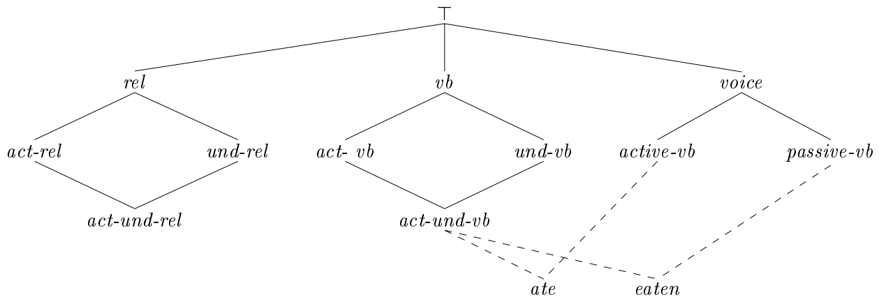
Figure 11: An illustration of multiple inheritance of lexical constraints
