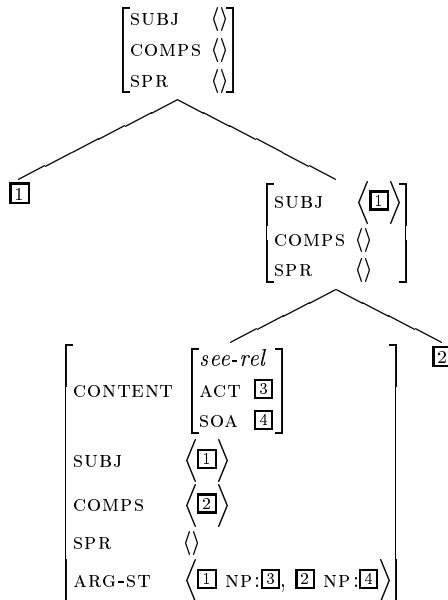
Figure 3: A simple example of the effects of the Valence Principle
