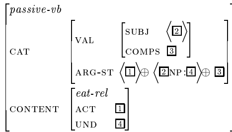
Figure 12: The passive form ‘eaten’
