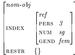
Figure 1: The semantic contribution of ‘she’
