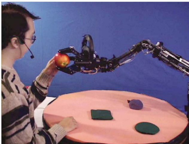
Fig. 9. Ripley is a 7 DOF manipulator robot terminating in a gripper, pictured here handing an apple to its human partner. The human speaks into a head-worn microphone to communicate with the robot. Two video cameras and touch sensors are mounted on the robot's gripper. Each actuated joint contains both a position and a force sensor, providing proprioceptive sensing.
