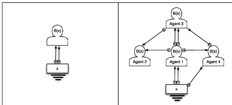
Fig. 17. Social belief networks.
