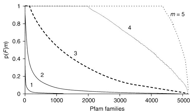
Fig. 4. The posterior probability of a correct classification into a given Pfam-A family F , given that the query sequence has m common 4-grams with the probe vector that represents the particular family. The x axis refers to the 5174 Pfam-A domain families rank ordered in decreasing probabilities. Results are shown for five cases, m = 1 \dots 5 . Correct classification reaches the 90% level when the number of 4-grams in common reaches five.
