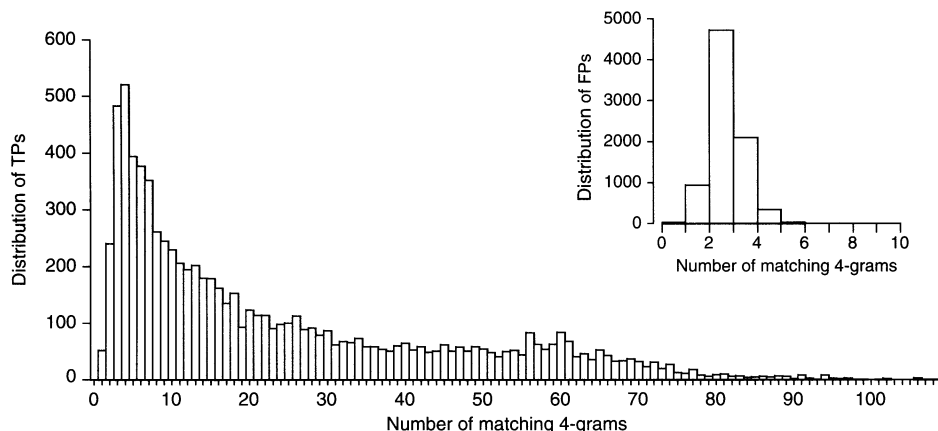
Fig. 5. Distribution of true positives (TPs) as a function of the number of matching 4-grams between the 4-gram vectors of the query sequence and the family probe vectors. The inset shows the distribution of false positives (FPs) as a function of the number of matching 4-grams. The distributions are generated by randomly sampling the 327 741 TPs and 147 176 FPs obtained from the application of a 4-grams-based family classification jackknife test to half of the Pfam-A sequences, the other half being used for defining/training the probe vectors of the Pfam-A families.
