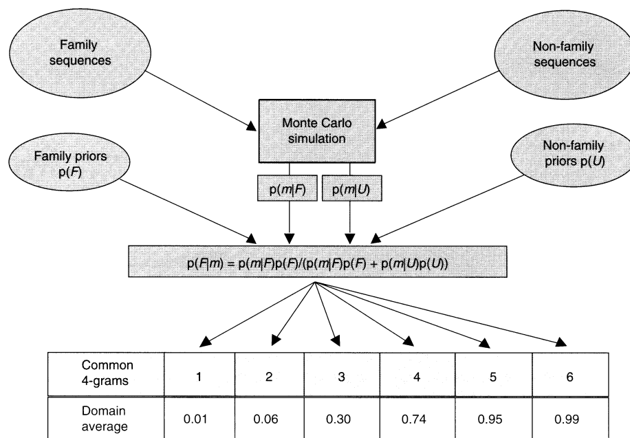
Fig. 3. Schematic description of the Monte Carlo calculations for determining the conditional probability, p(F|m) , of family F , also called probe certification value, given m common n -grams between the probe and query sequence.
