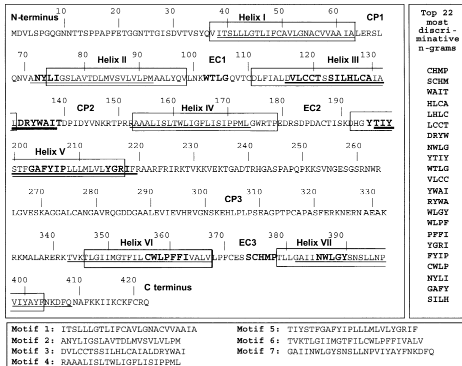
Fig. 7. Distribution of 4-grams (bold letters) in the human serotonin receptor (ID: 5h1a_human) in comparison with the position of PRINTS motifs (underlined) and transmembrane helices (boxes). Extracellular loops are indicated by the N-terminus and EC1 to EC3, cytoplasmic loops are indicated by the C-terminus and CP1 to CP3. The seven transmembrane helices are indicated as helix I to helix VII. The 4-grams shown are the top 22 most strongly contributing to the classification. They are also listed on the right of figure, rank ordered by weight. The motifs from the PRINTS database ( http://bioinf.man.ac.uk/dbbrowser/PRINTS ) are listed at the bottom of the figure.
