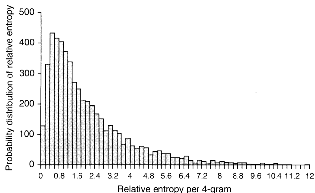
Fig. 2. Probability distribution of the relative entropy per 4-gram for the 5193 families in Pfam-A. There is a significant gain in information for the majority of family distributions compared with the background distribution. The mean value is calculated to be 2.072, indicating that the preferences for the 4-grams in the Pfam families are about 2 orders of magnitude different from those in the background distribution. Note that the information gain per sequence is the x axis multiplied by the sequence length, because the results are normalised with respect to sequence lengths (i.e. divided by the total number of n -grams in each sequence).
