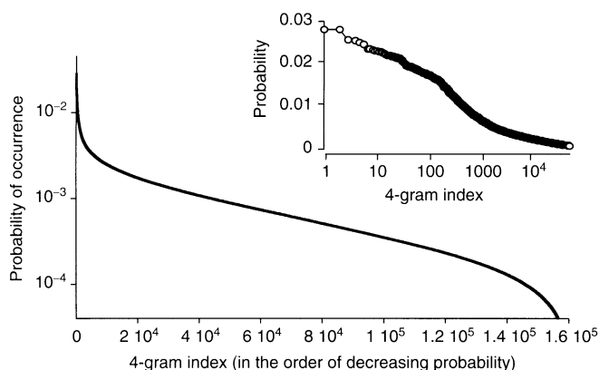
Fig. 1. Probability of occurrence of all the 4-grams in Pfam-A. A total of 159 996 unique 4-grams were found in 975 024 domain sequences. The 4-grams are displayed in rank order by decreasing probability, piU . piU is below 0.25% for a large majority of 4-grams. The inset displays the subset of the most probable 4-grams. The most common 4-grams occurred in less than 3% of sequences. This suggests that the probability of finding a large number of matching 4-grams in unrelated sequences is low.
