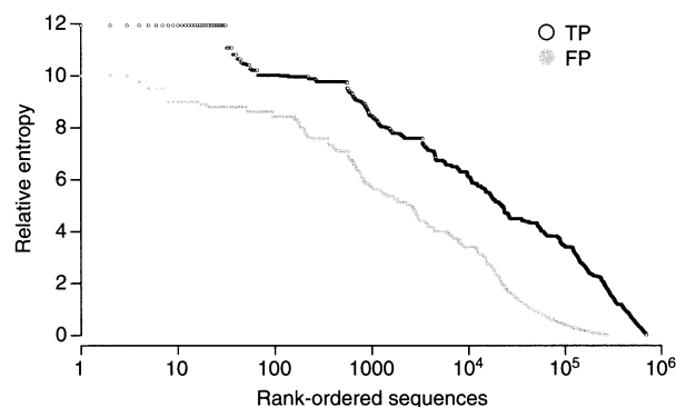
Fig. 6. Comparison of the relative entropy per 4-gram of the true positives (TPs) and false positives (FPs). FPs with high values suggest distributions that might be exploited by breaking families into subclasses and creating probes with greater specificity.
